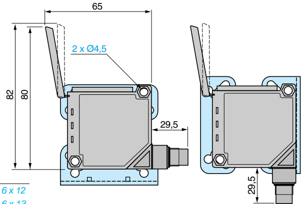
Fixing bracket mounting according to position of connector (1)
