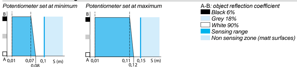
With reflector XUZC50 Object 10 x 10 cm; 1 White 90%; 2 Grey 18%
