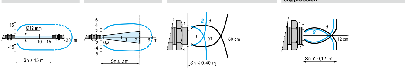
With reflector XUZC50 Object 10 x 10 cm; 1 White 90%; 2 Grey 18%
