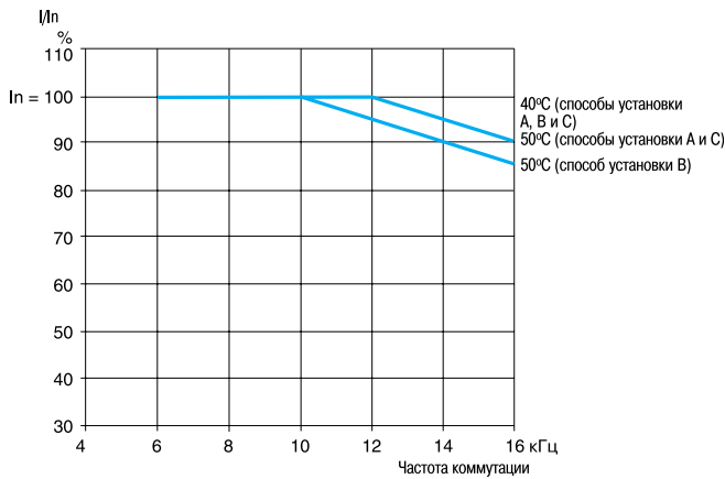
ATV 21HU30N4
