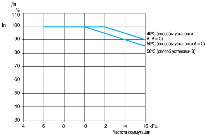
ATV 21HU30M3X
