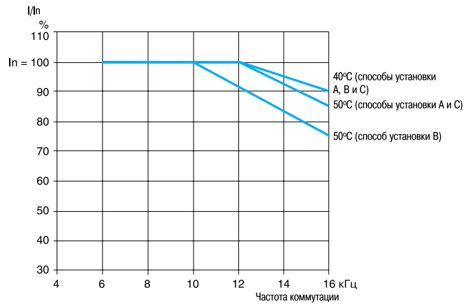
ATV 21HU40N4
