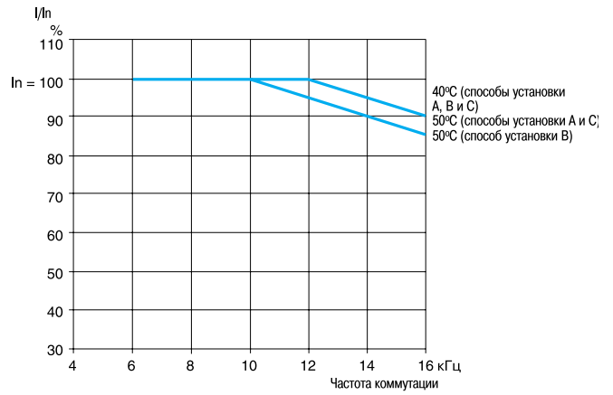
ATV 21HU75N4
