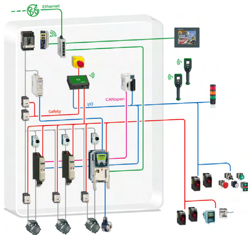
A complete ready-to-use-architecture for self-erecting cranes; related/available software functions: Data storage monitoring, wind speed control, smooth slewing, and safety solutions.
