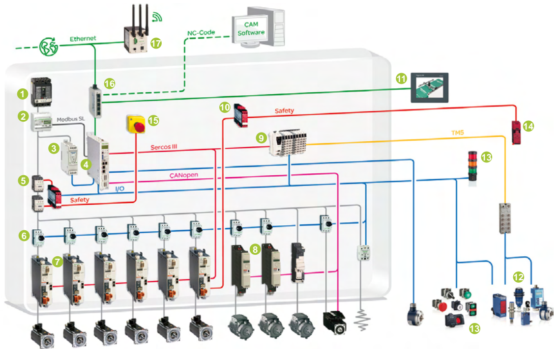
Compact / Sercos / Motion Controller LMC078
