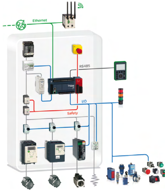
Booster multidrive architecture for typical booster solutions for fresh water supply of large buildings, e.g. hotels, office buildings, shopping malls, service areas, resorts, etc.
