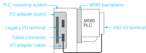
The I/O Wiring System adapts Legacy I/O Terminals to X80 I/O
