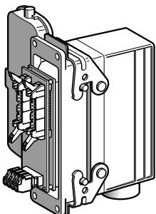
ABE-7ACC80 + ABE-7ACC81
