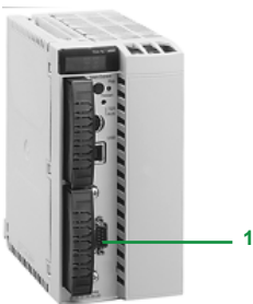
TSX P57 454/554M
