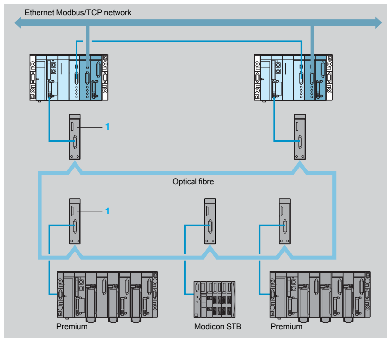
1 OZD FIP G3 fibre optic transmitter (see page 5/109)
