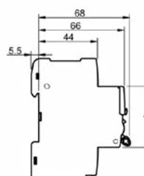
iOF+SD24 (A9A26897)
