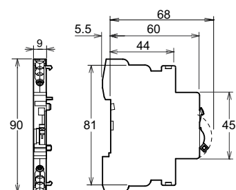
OF+SD/OF
