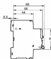
iOF+SD24 (A9A26898)
