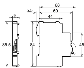
OF+SD24
