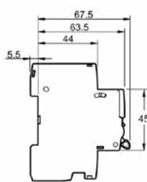
iOF, iSD
